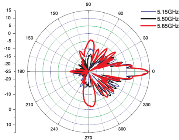
V-Plane Co-polarization pattern
