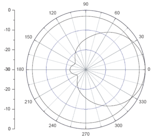
H-plane Co-polarization Pattern
