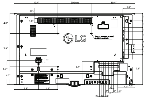
65SE3KB Rear Jack Pack
