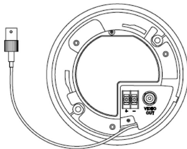
Rear View of Dome Base
