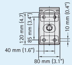
Back side of wall mount bracket
