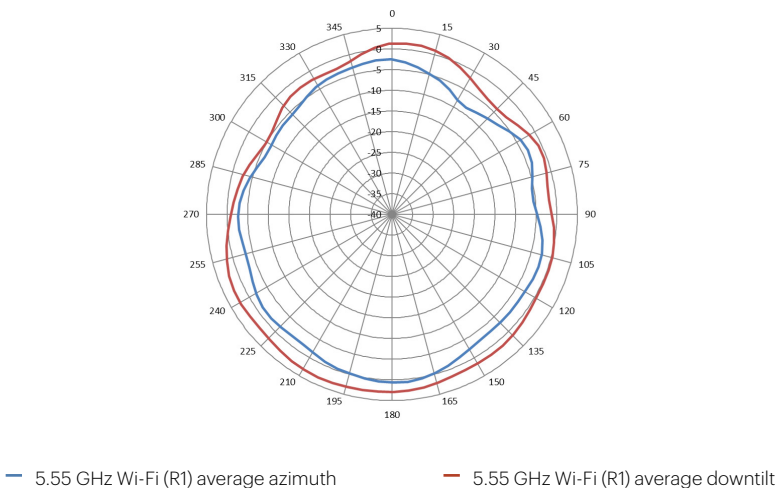
Figure 2. 5.55 GHz Wi-Fi antenna patterns (horizontal)
