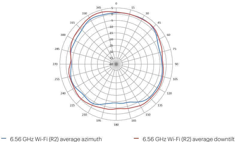
Figure 3. 6.56 GHz Wi-Fi antenna patterns (horizontal)
