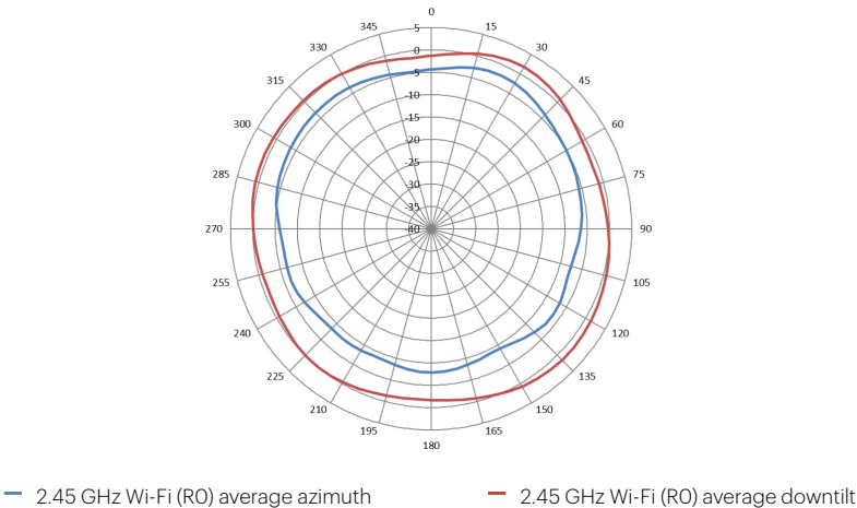
Figure 1. 2.45 GHz Wi-Fi antenna patterns (horizontal)
