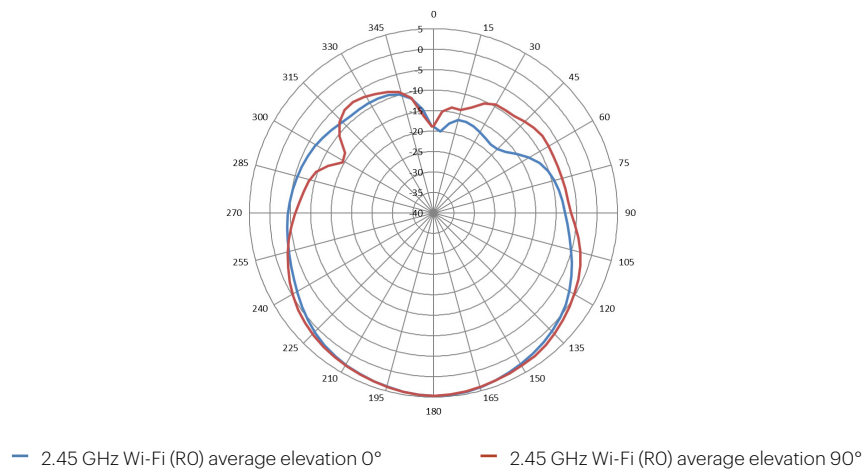
Figure 4. 2.45 GHz Wi-Fi antennas patterns (vertical)
