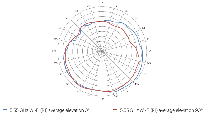
Figure 5. 5.55 GHz Wi-Fi antenna patterns (vertical)
