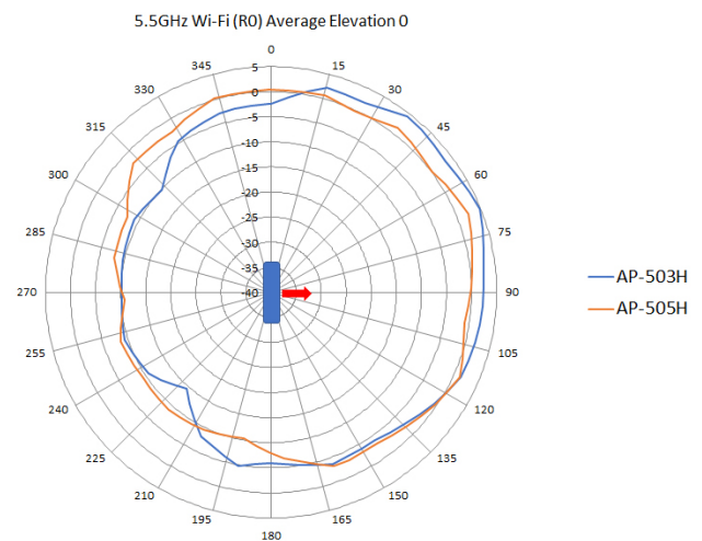
5.5 GHz Wi-Fi (antennas 0, 1)
