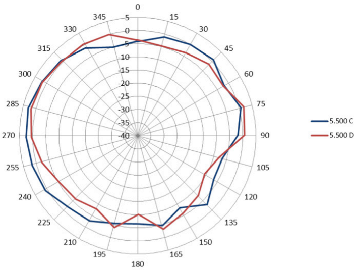
Elevation plane (front view) 5.500 GHz
