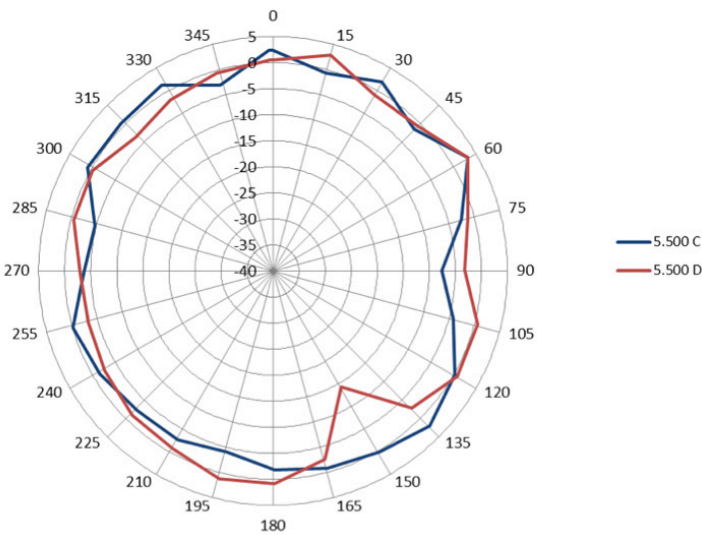
Horizontal or azimuth plane (top view) 5.500 GHz
